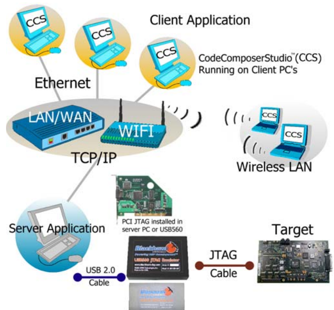
Blackhawk PCI or USB560 Emulator Installed on Server
